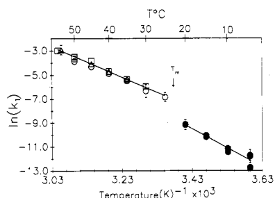
FIGURE 3: Arrhenius plot of DMPC desorption rates from DMPC LUV. Each point represents the result of one exchange experiment, and each has a calculated uncertainty. A few are shown; many are smaller than the symbols. Different symbols represent different vesicle preparations used in similar experiments. The two distinct lines represent sets of experiments performed above and below the phase transition temperature ( T_m ) of 23 °C. Each distinguishable point below T_m actually contains two identical experiments run simultaneously. At various times, aliquots were eluted over an ion-exchange column as described in the text, and the ^3\text{H} and ^{14}\text{C} in the donors were determined. A total of 12–20 points were taken for each experiment.
